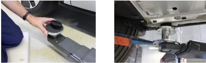
The ATS support plate system with form-fit vehicle adapters in use Photos: MAHA
